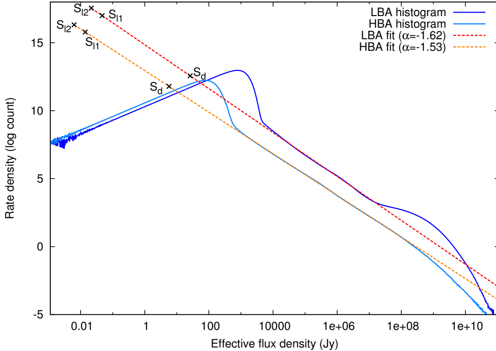
Figure 9. Observed LBA distribution after band-pass correction and flux calibration. S_{11} and S_{12} denote the limits of the distribution with a sharp lower cut-off (Eq. (18)) and uniform lower limit (Eq. (19)), S_d is the average lower limit of RFI that is detected.
